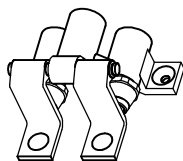
FOOT VALVE Assembly,color-coded dual pedals,self closing valves,for use with spout bases.Two 1/2"NPT female iniets and one 1/2"NPT female outlets.Rough chrome valve body with polished chrome foot pedal.
