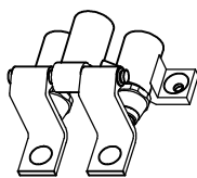
FOOT VALVE Assembly,color-coded dual pedals,self closing valves,for use with spout bases.Two 1/2"NPT female iniets and one 1/2"NPT female outlets.Rough chrome valve body with polished chrome foot pedal.
